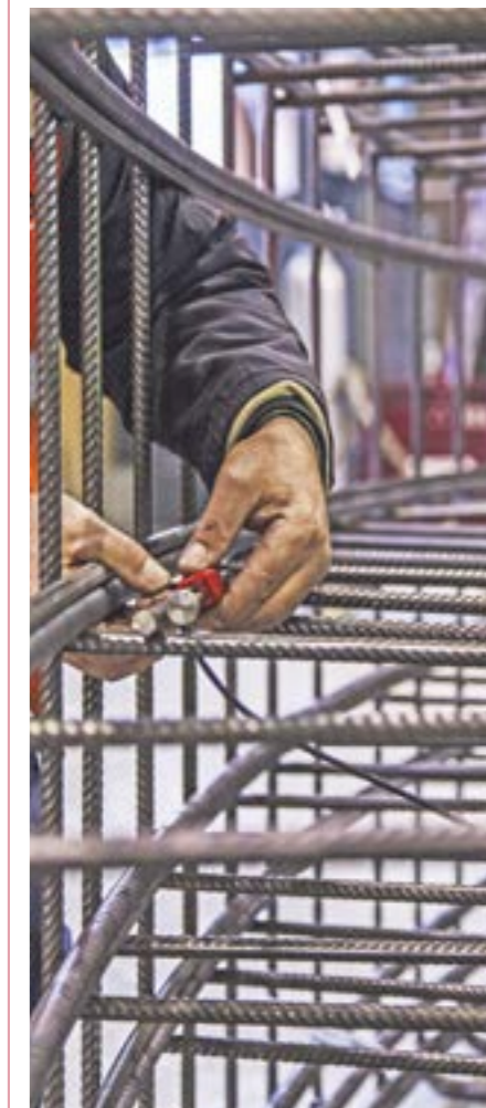
TELT - Tunnel Euralpin Lyon Turin, installation of VW strain gauges within TBM precast concrete element.
